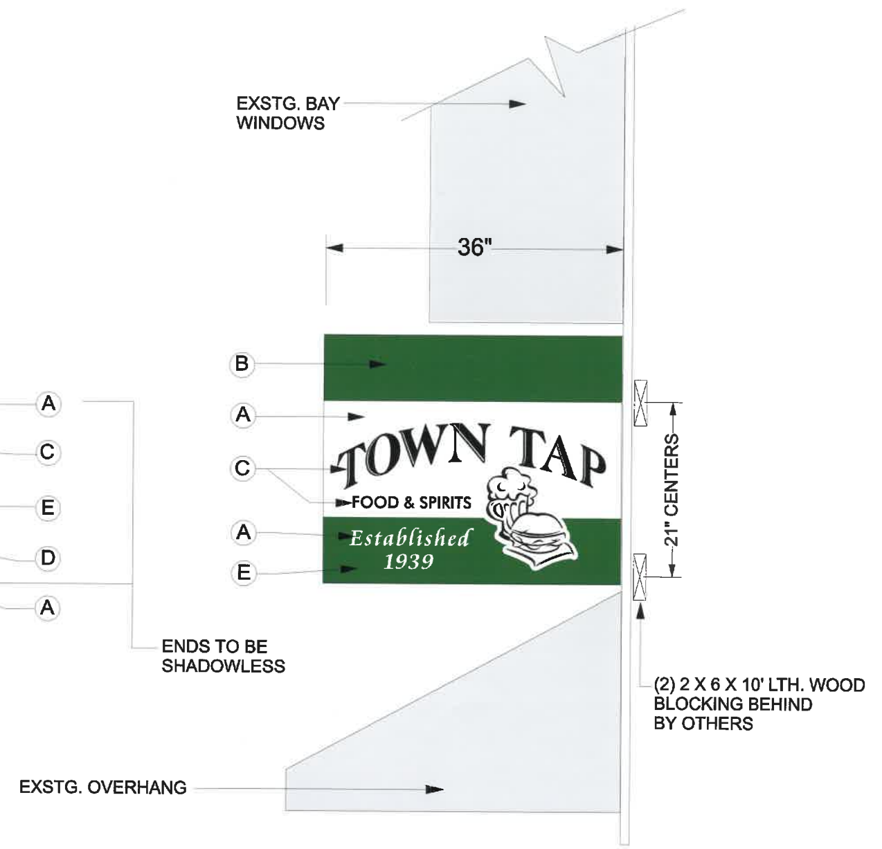
END VIEW
